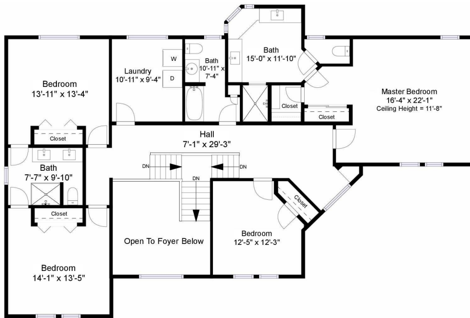
Second Floor Plan Ceiling Height = 8'-0"
