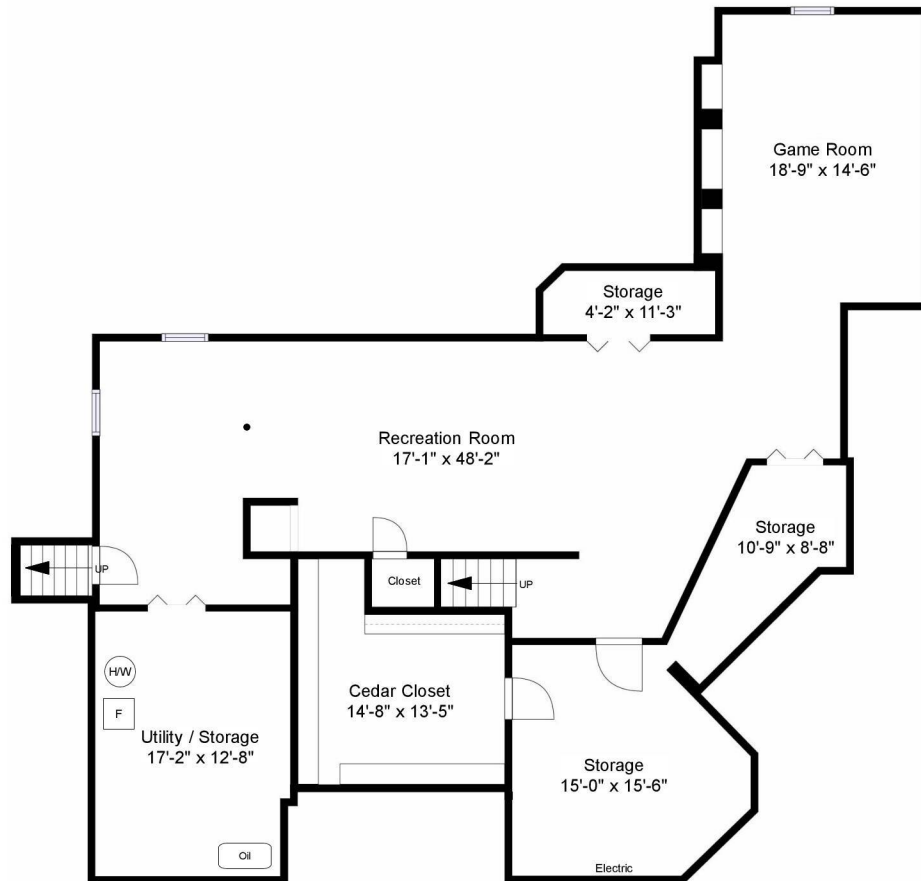
Lower Level Plan Ceiling Height = 6'-10"
